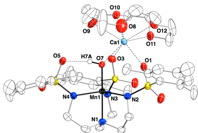
Figure 5. Molecular structure of [\text{Ca}^{\text{II}}(\text{OH})\text{Mn}^{\text{III}}]^+ complex.
