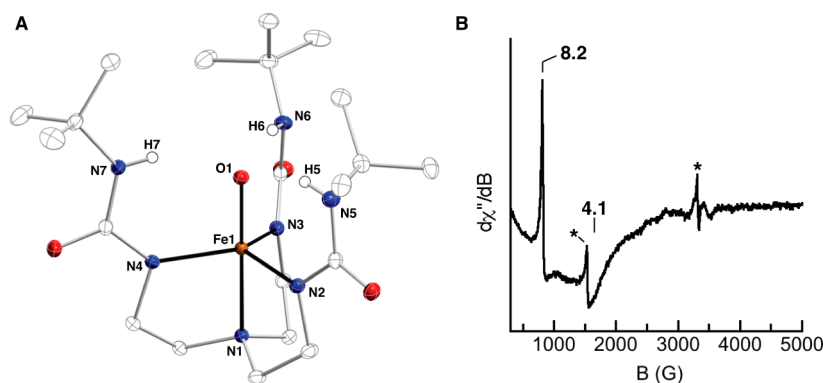
Figure 3. Molecular structure (A) and EPR spectrum of [\text{Fe}^{\text{IV}}\text{H}_3\text{buea}(\text{O})]^- (B). Asterisks in panel B indicate signals from small amounts of impurities.
