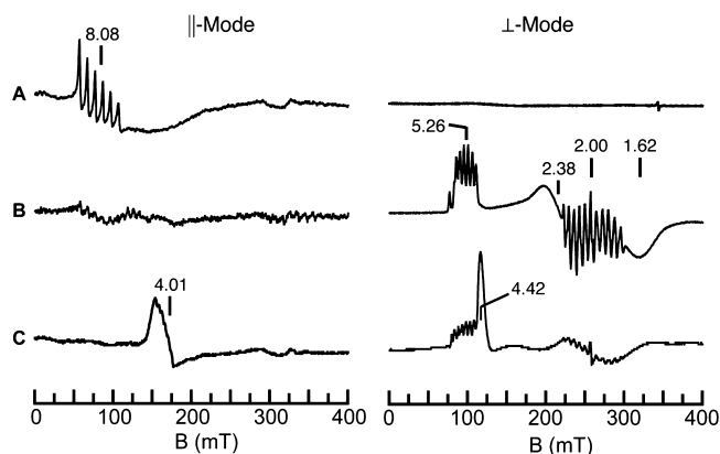
Figure 4. EPR data for the stepwise oxidation of [\text{Mn}^{\text{III}}\text{H}_3\text{buea}(\text{O})]^{2-} (A) to [\text{Mn}^{\text{IV}}\text{H}_3\text{buea}(\text{O})]^- (B) and [\text{Mn}^{\text{V}}\text{H}_3\text{buea}(\text{O})] (C). The signal at g = 4.4 in trace C is unreacted [\text{Fe}^{\text{III}}\text{Cp}_2]^+ .
