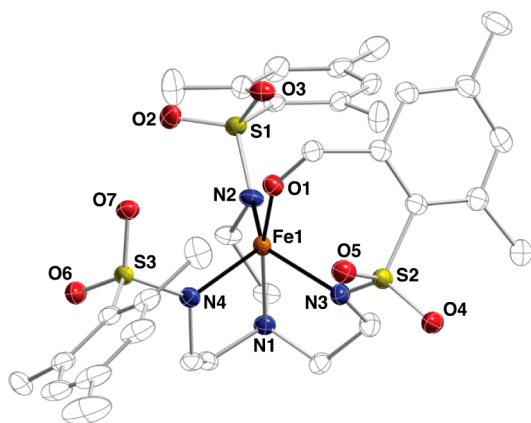
Figure 7. Molecular structure of Fe III -alkoxide product from oxidation of [NMe 4 ][Fe II MST] with NMO.
