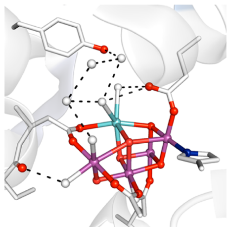
Figure 1. Structure of the OEC cluster (PDB 3ARC) illustrating the H-bonding network (dashed lines). Sphere key: purple (Mn), light blue ( \text{Ca}^{2+} ), red (oxido/hydroxo ligands), blue (nitrogen), white (water).
