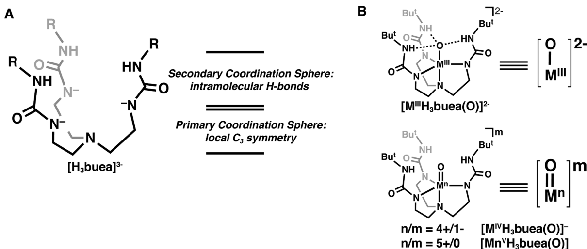
Figure 2. Depiction of a (A) H-bonding ligand and (B) \text{M} -oxo complexes ( \text{M} = \text{Fe}, \text{Mn} ).
